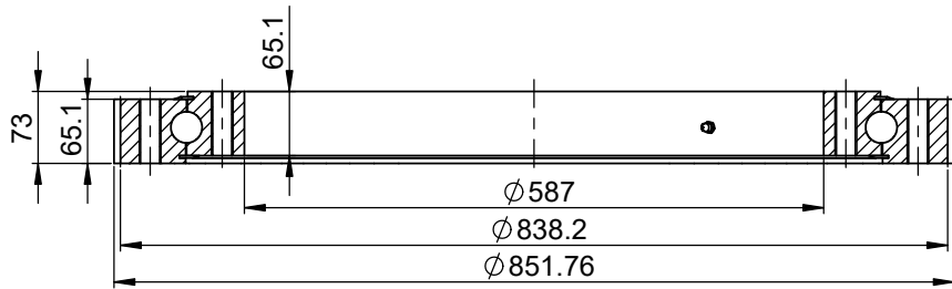
VIEW F-F
